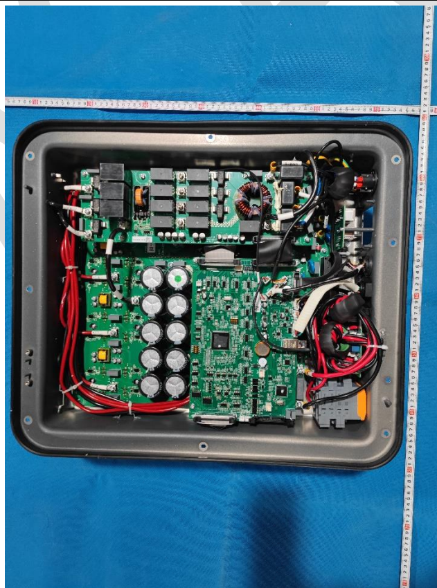
Internal view
